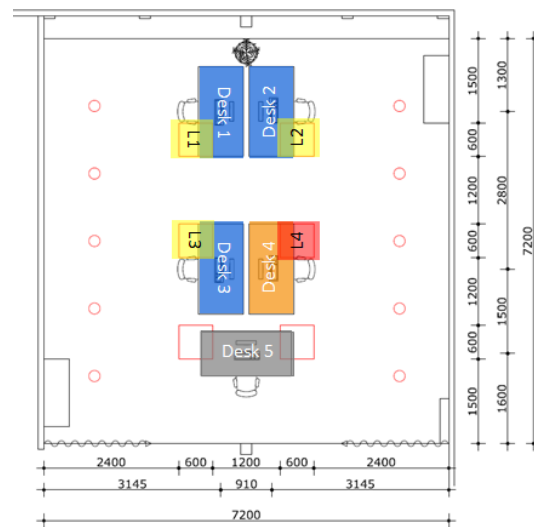
Fig. 2: Plan view of the experiment room.
