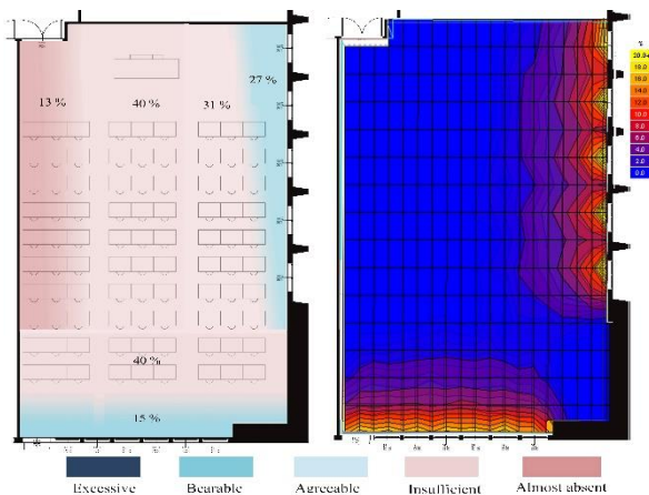
Fig. 5: Index of Dissatisfaction and DA_{500} values
