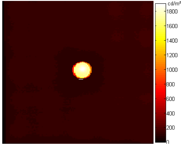
Fig 1: Luminance map of an arbitrary stimulus: a central zone of uniform high luminance level with a uniform low luminance surround.
