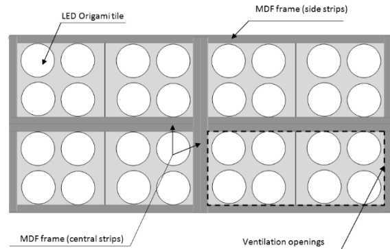
Fig. 1: Rear view illustration of the 2 \times 4 Origami BPG762 arrays in the prototype; taken from Mangkuto et al. (2014)
